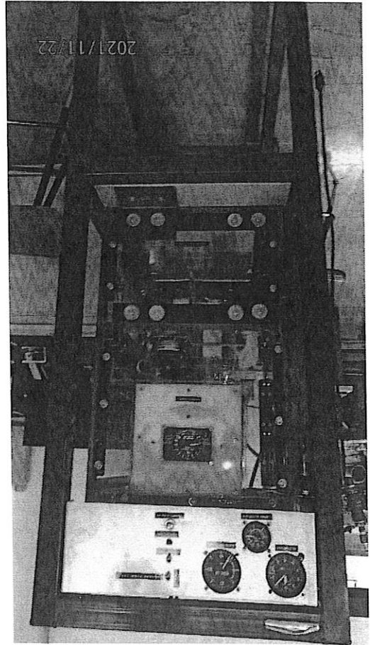
TAG# 173108 AVIATION EQUIPMENT: CABIN ATMOSPHERIC/PRESSURIZATION MOCK-UP
