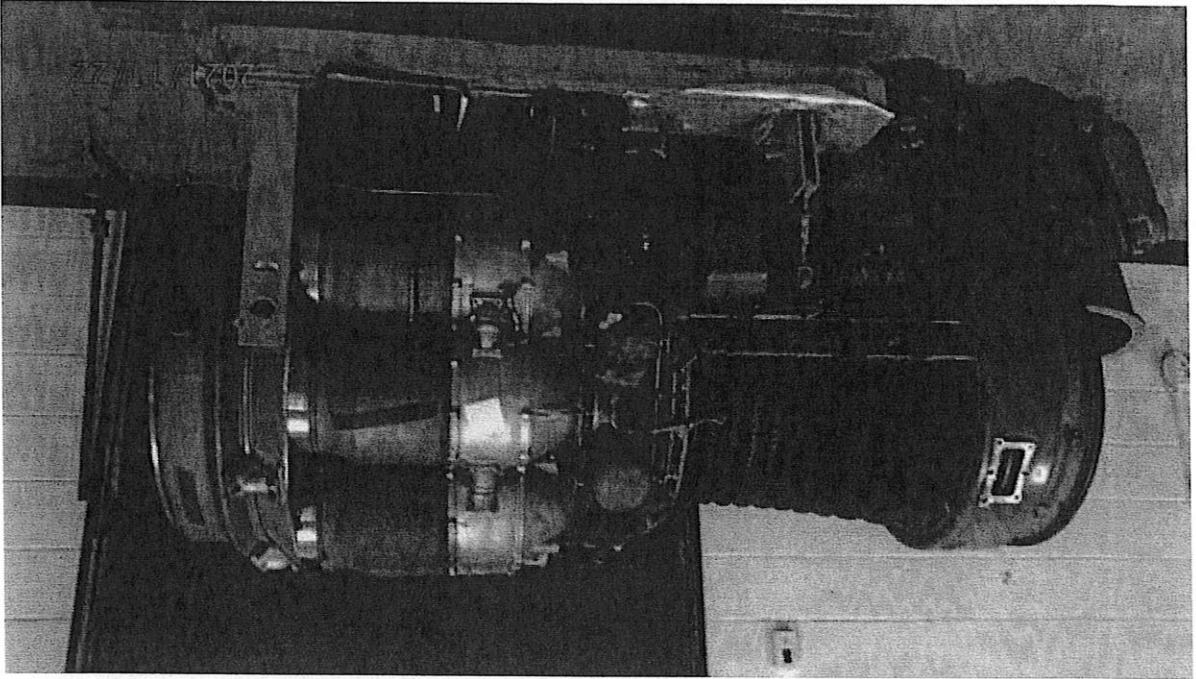
TURBINE ENGINE – ROLLS ROYCE AVON RA-7
